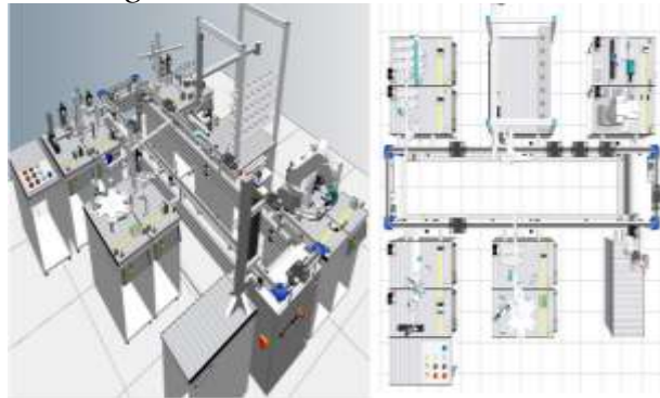
Figure 1: MPS 500 - FSM Station
