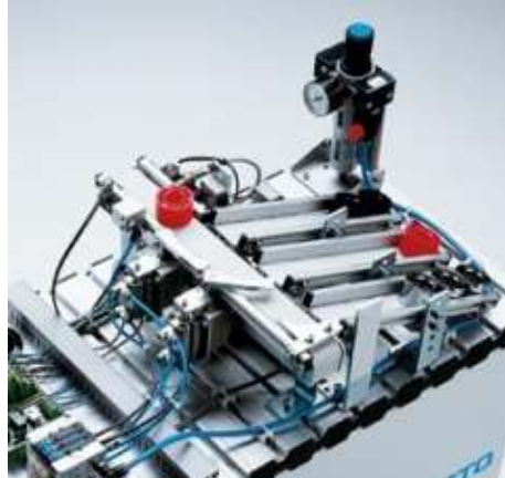
Figure 2: Sorting station
