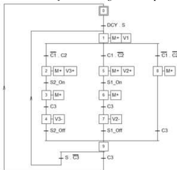
Figure 3: GRAFCET of the sorting station operation
